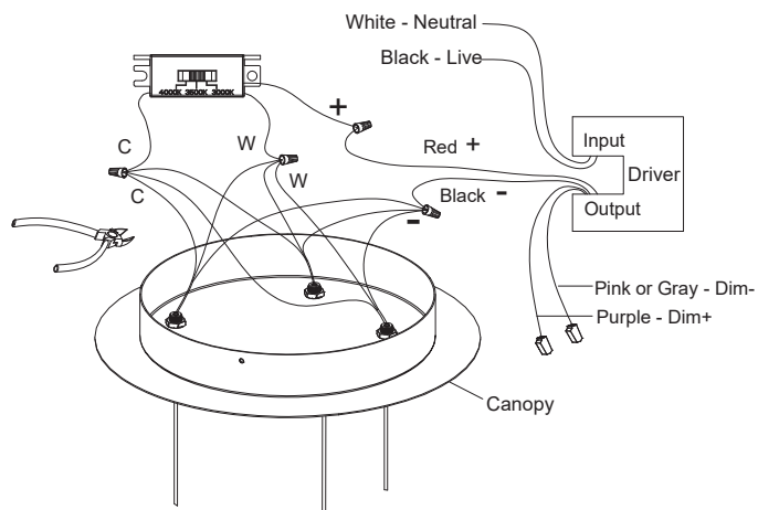
Fig. 2 Wire Diagram
