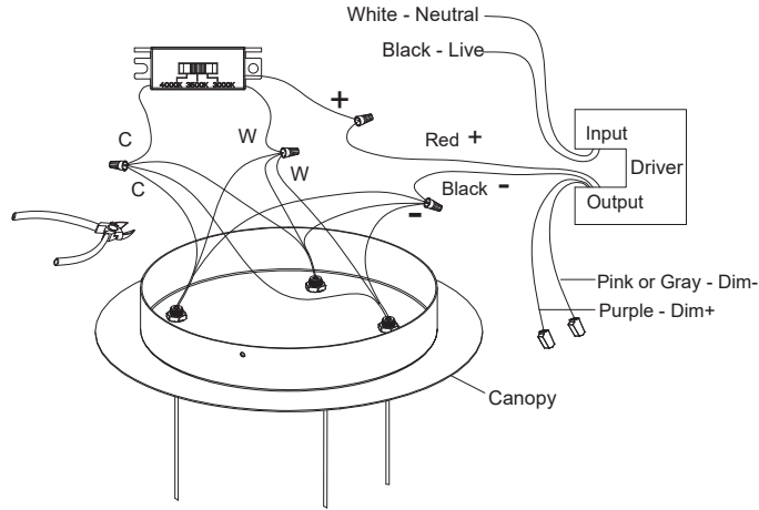
Fig. 2 Wire Diagram
